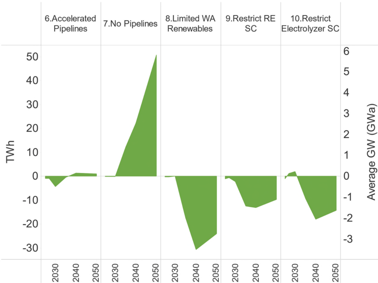
Washington Electrolysis Electricity Demand relative to Core Case (TWh)
