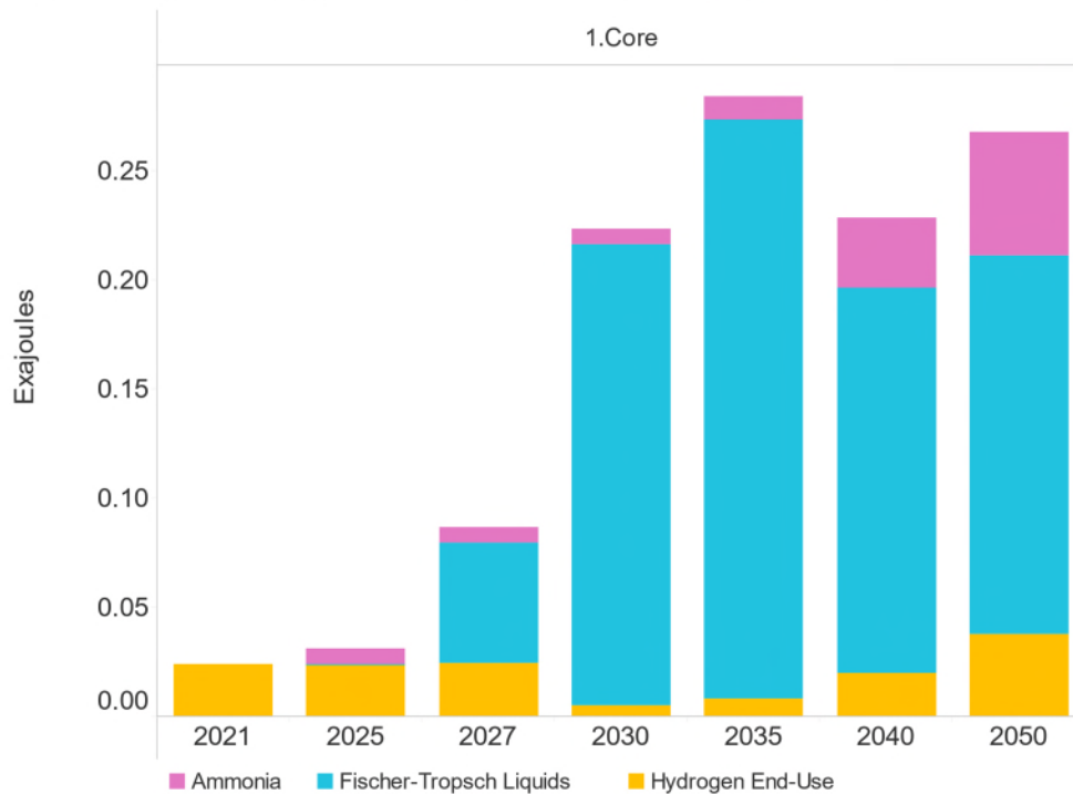
Hydrogen and Hydrogen-Derived Fuels Consumption in WA
